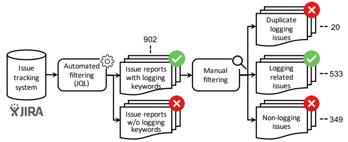
Fig. 3. Our process of collecting logging-related issue reports.
