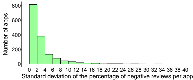
Fig. 6: A histogram of the standard deviation of the percentage of negative reviews per app
