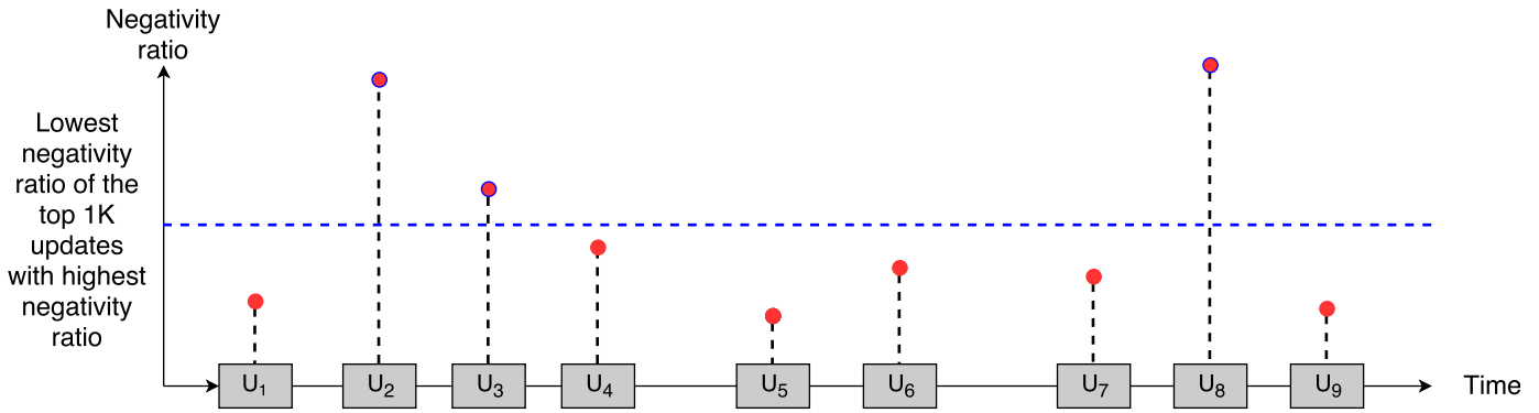
Fig. 4: An example of an app with nine updates U_1 to U_9 . The blue dotted line in the figure shows the lowest negativity ratio of the top 1,000 updates with the highest negativity ratio. In our study, we included both updates U_2 and U_8 as they are separated by other updates while we excluded update U_3 since it follows the bad update U_2
