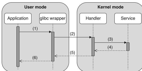
Fig. 1 The sequence of a system call
