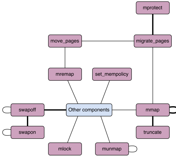
Fig. 11 All race conditions for memory management system calls (the purple nodes) that were fixed during the last decade. The thick lines indicate two fixed race conditions
