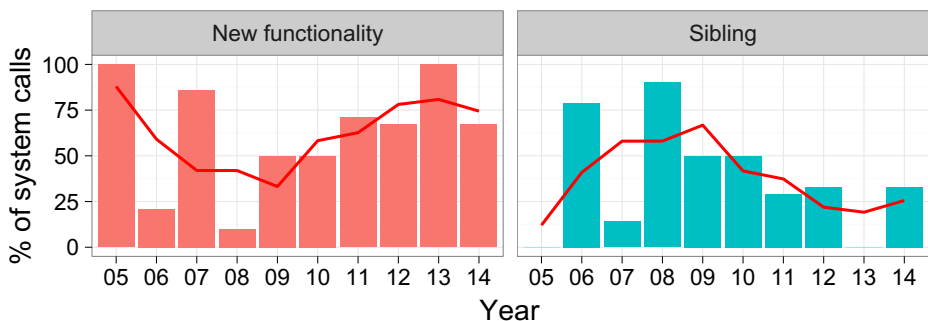
Fig. 4 The percentage of new system calls that provide new functionality and the number of sibling system calls. The red line is a LOESS regression fit line (Fox and Weisberg 2010)
