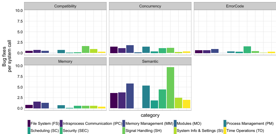
Fig. 10 The number of bug fixes per system call in each bug category over the last decade
