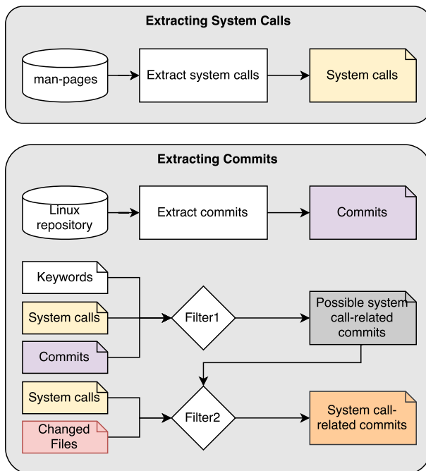
Fig. 2 An overview of our data collection
