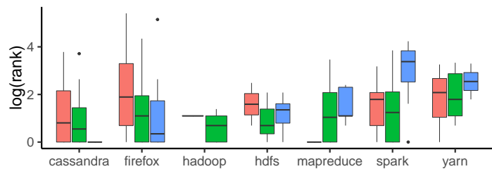
Fig. 7. Rank (In log scale) at which ConfigMiner reports the appropriate options for each of the 3 categories of questions.
