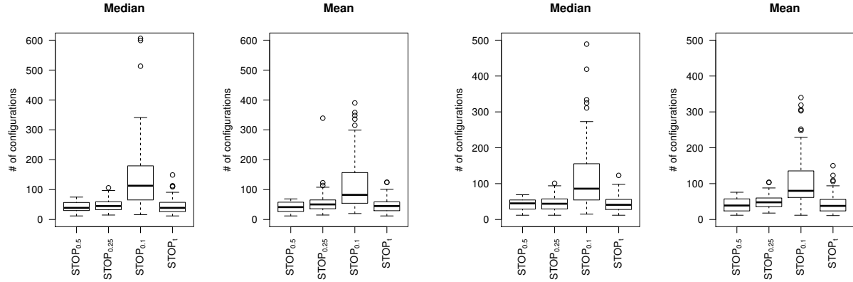
(a) Spring PetClinic
