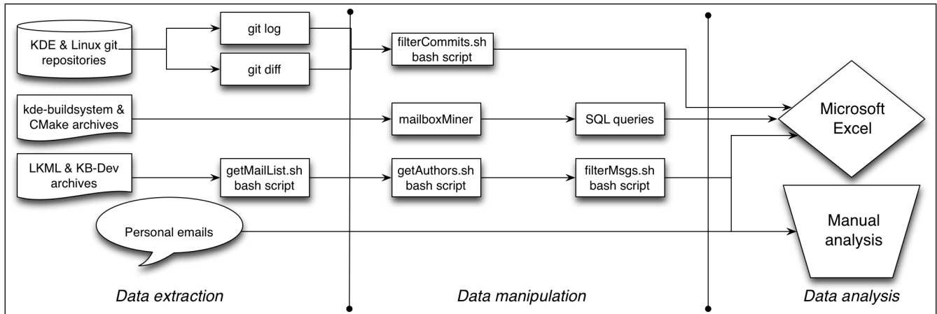
Figure 2. Summary of the data extraction, manipulation and analysis process.
