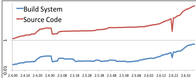
Figure 1. Evolution of Linux kernel source code, v. 2.4.0 to 2.6.39, with millions of LOC (logarithmical scale) plotted against time.
