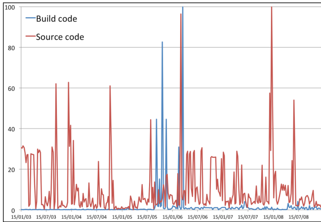
Figure 3. Normalized (maximum = 100%) weekly churn per file statistics for KDE build and source code. Note the peaks during the August 2005 - March 2006 migration period.
