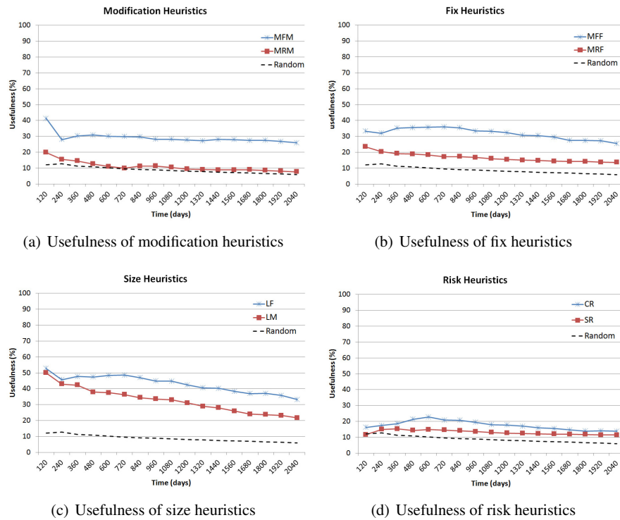
Figure 5. Usefulness of heuristics compared to the random heuristic for the Eclipse OSS system
