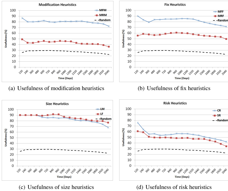
Figure 4. Usefulness of heuristics compared to the random heuristic for the commercial system
