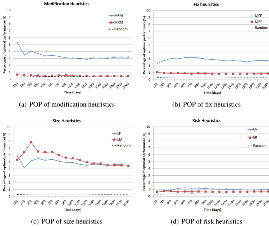
Figure 7. POP of heuristics compared to the random heuristic for the Eclipse OSS system
