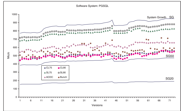
Figure 5: Authoritativeness comparison wrt PGSQL
