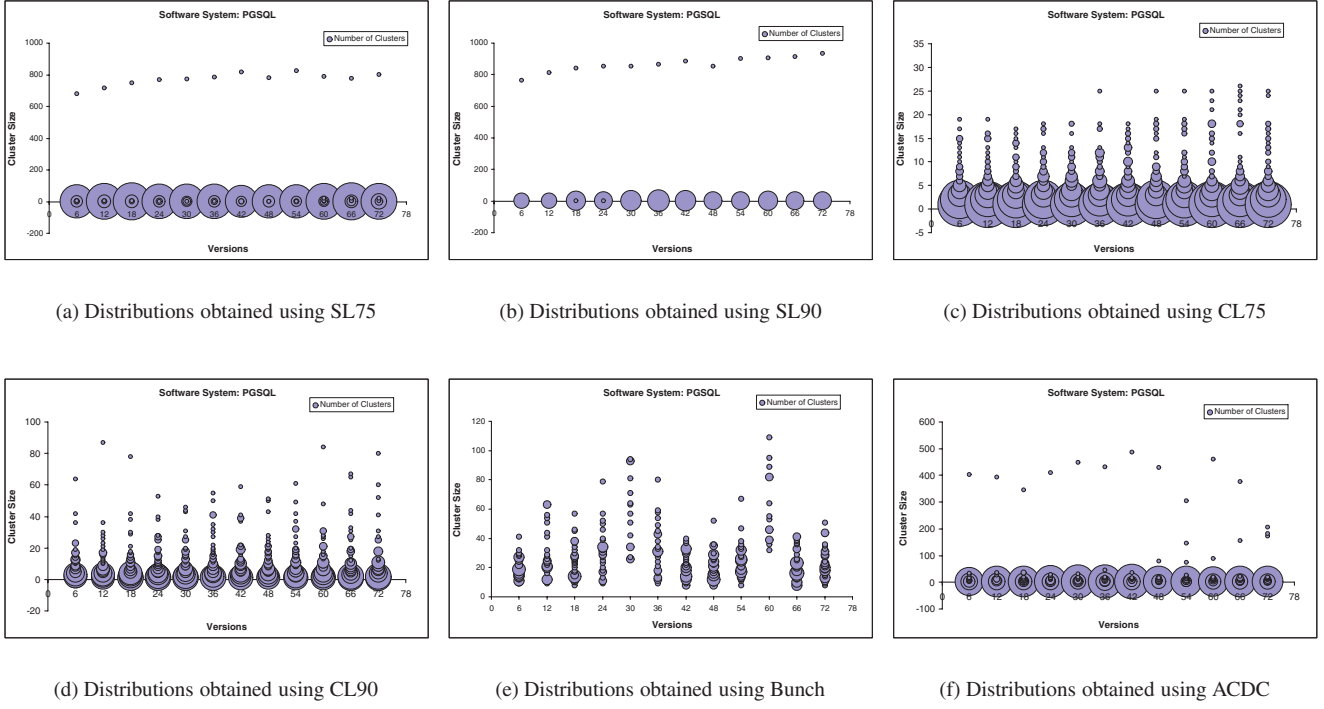
Figure 6: Bubble chart based distribution comparison of clustering algorithms wrt PGSQL
