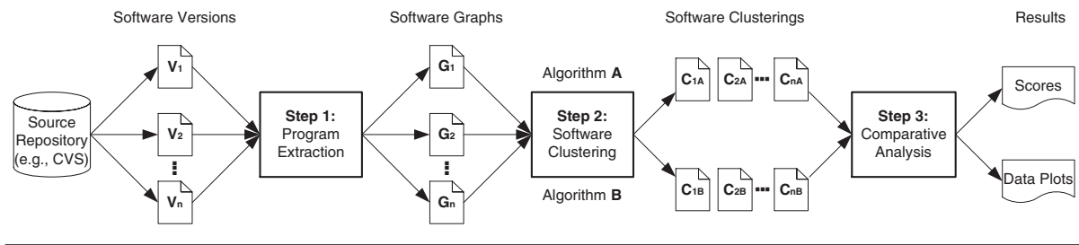
Figure 1: Comparative analysis of software clustering algorithms in the context of software evolution
