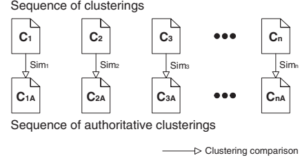
Figure 4: Inter-sequence clustering comparison
