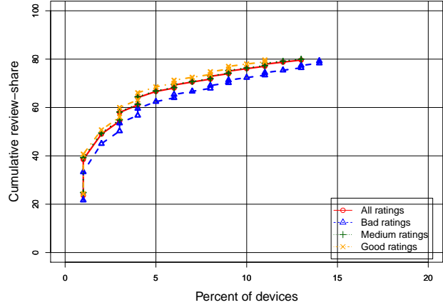
Figure 5: Percent of Android devices which contribute X% (X ranges from 0 - 80) of the reviews for all paid game apps
