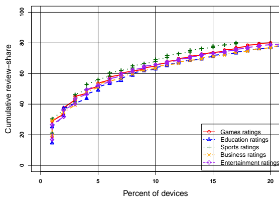
Figure 7: Percent of Android devices used to give X% (X ranges from 0 - 80) of the reviews of free apps in 5 categories
