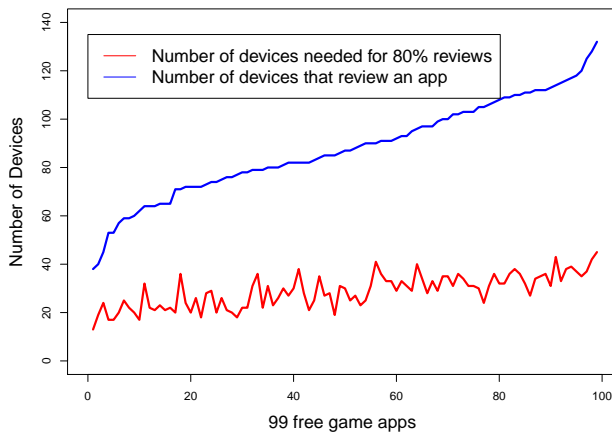
Figure 3: Number of Android devices that account for 80% of the reviews for each game app, compared with the total unique devices that review the app
