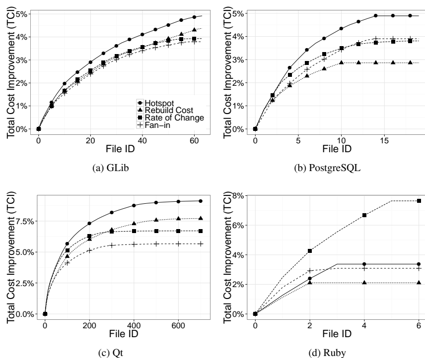
Fig. 7: Cumulative curves comparing the four approaches for selecting header files for build performance optimization. The Total Cost Improvement (TCI) measures the reduction of time spent rebuilding in the future (testing corpus) when the performance of the selected header files are improved by 10%.
