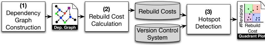
Fig. 3: Overview of our hotspot analysis approach.
