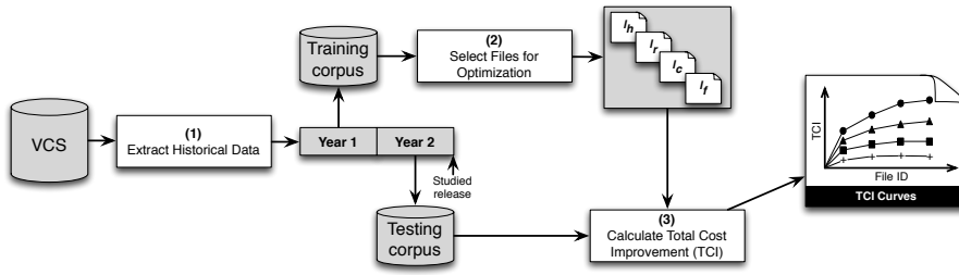
Fig. 6: Overview of our simulation exercise.
