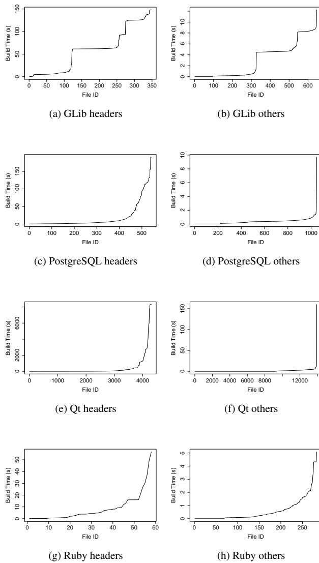
Fig. 4: The rebuild cost of the header and other (primarily source) files in the studied systems.
