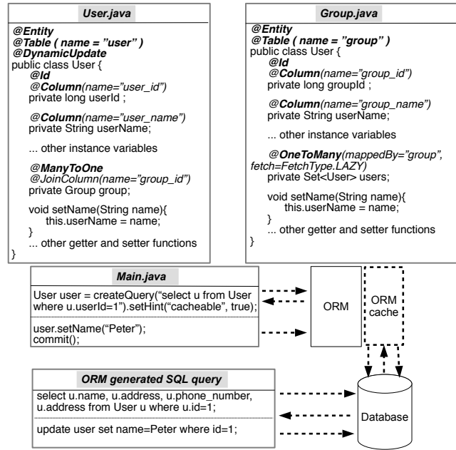
Figure 1: Example of database entity classes and how ORM translates object manipulation to SQL queries.
